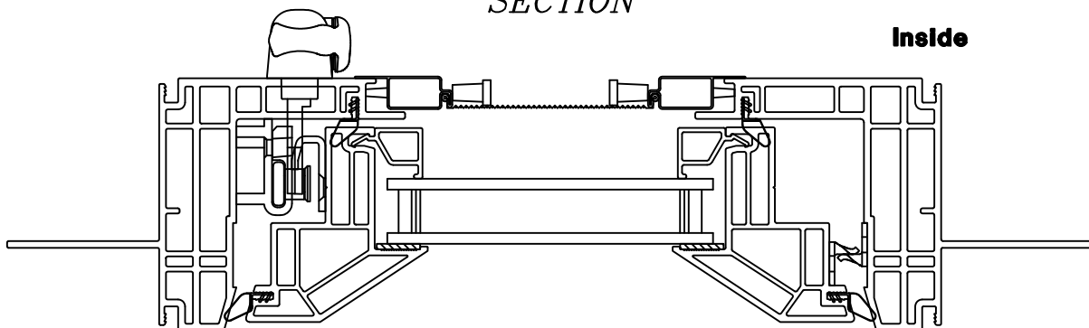
HORIZONTAL SECTION
