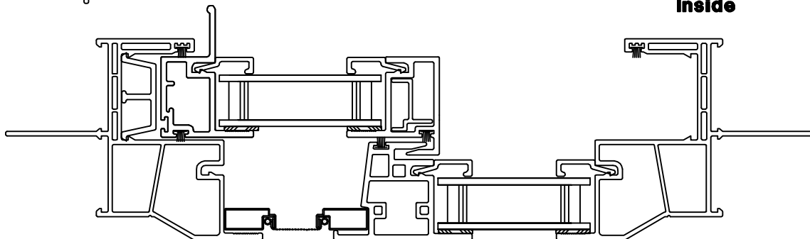
HORIZONTAL SECTION
