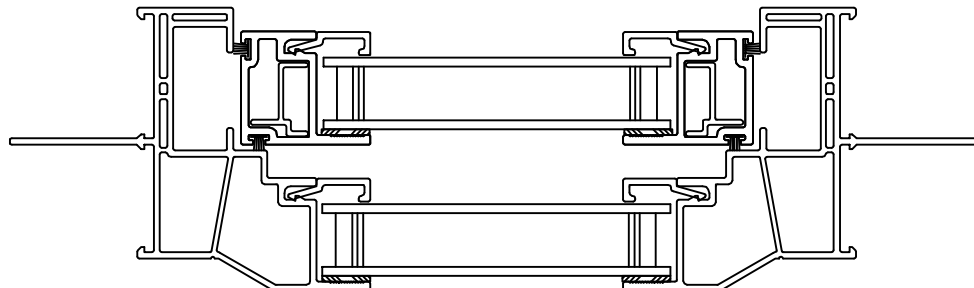
HORIZONTAL SECTION
