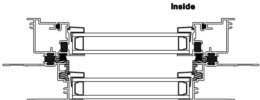
HORIZONTAL SECTION
