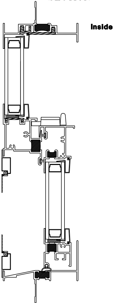
VERTICAL SECTION
