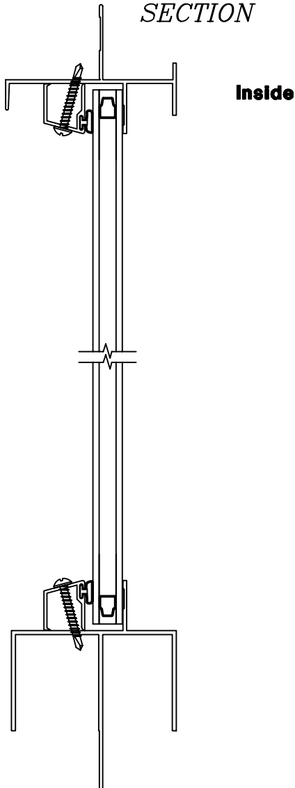
HORIZONTAL SECTION
