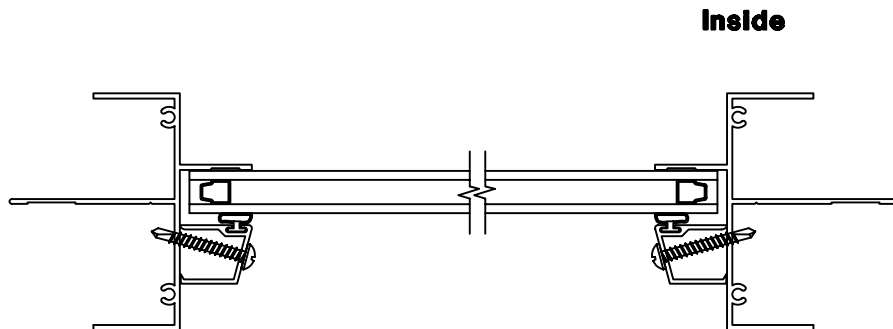
HORIZONTAL SECTION
