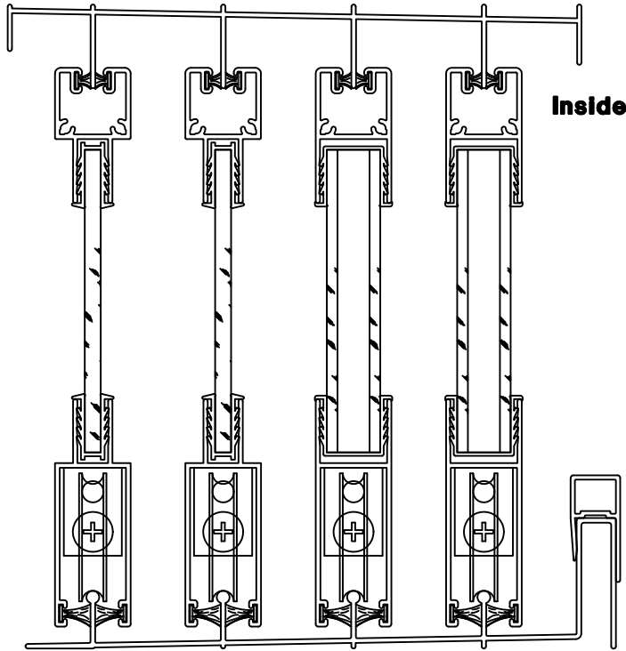
HORIZONTAL SECTION
