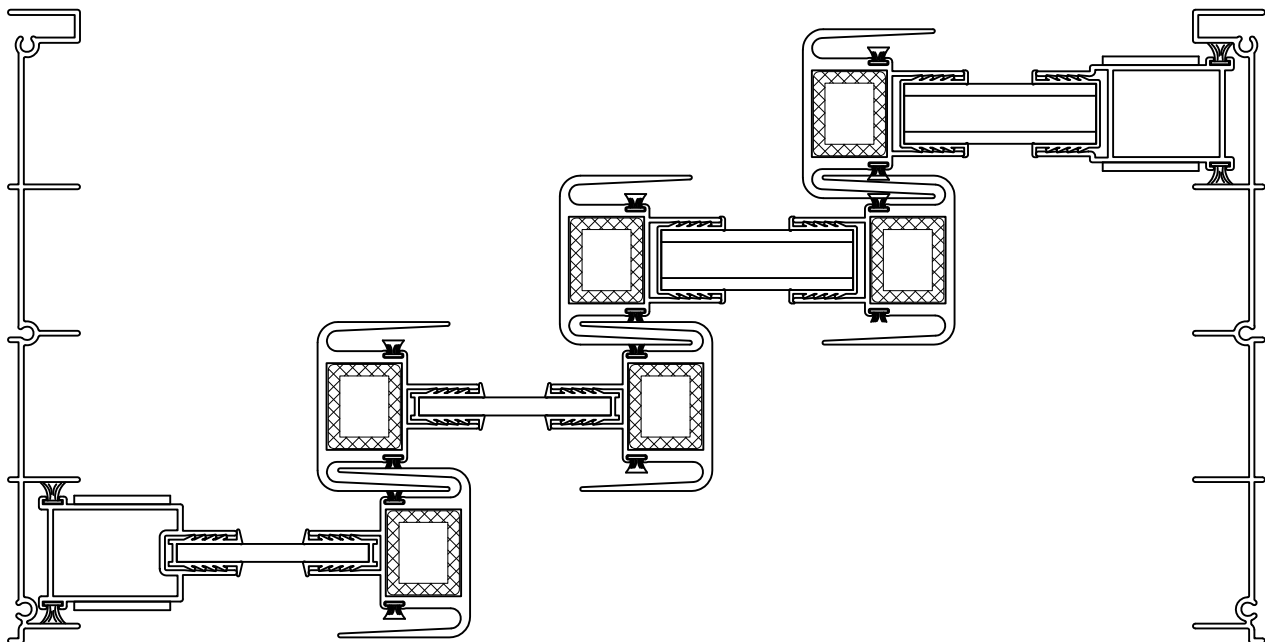
HORIZONTAL SECTION
