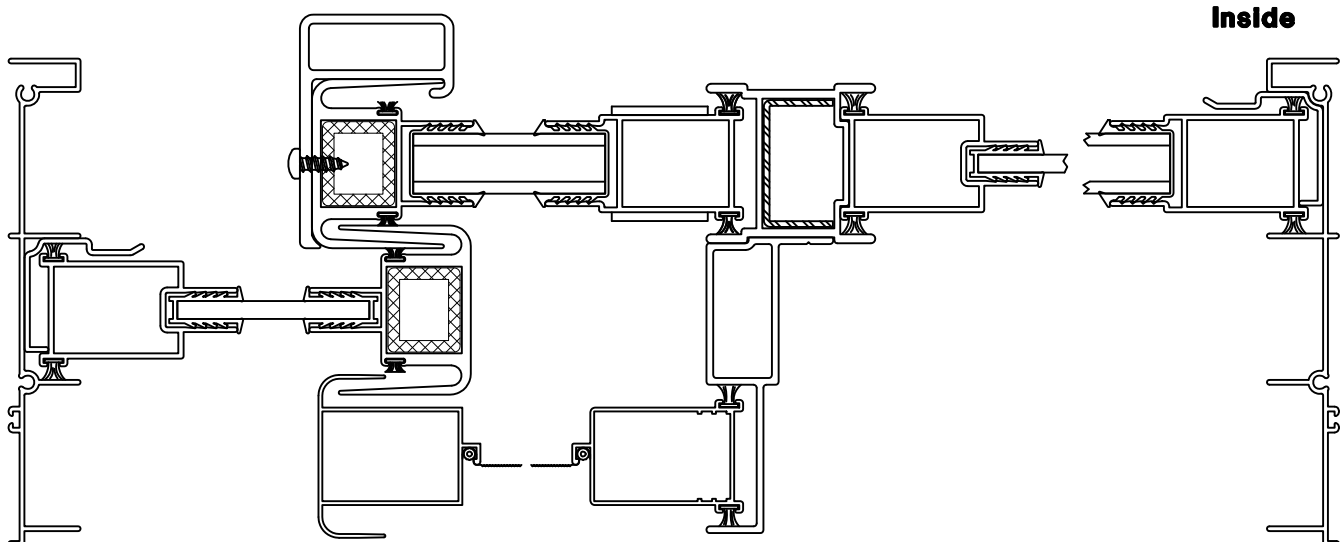
HORIZONTAL SECTION
